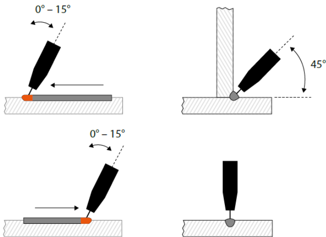
Fig. 6. Welding technique
