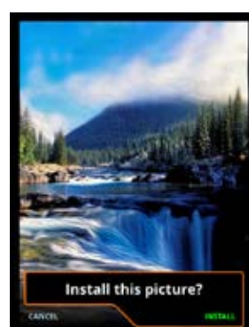
Personalized screensaver
